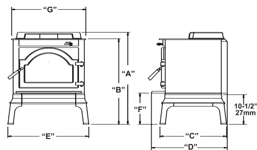
Wood Stove with Legs
