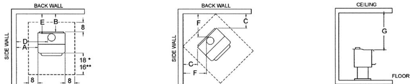
CLEARANCES TO COMBUSTIBLES
