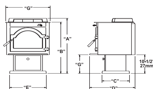
Wood Stove with Pedestal
